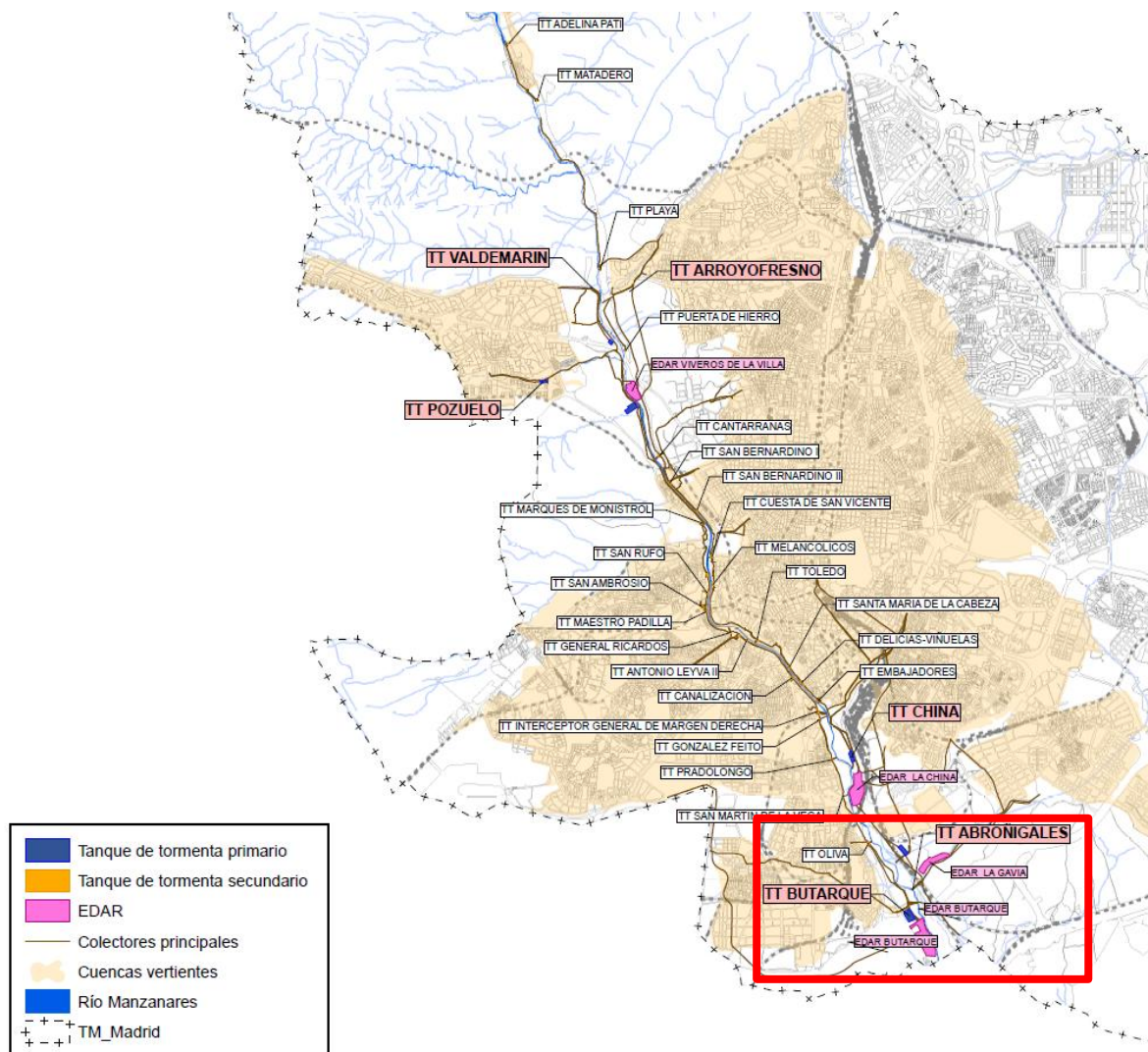
Figure 1 : Manzanares system overview with the location of the main sewers, main and secondary detention tanks and WWTP. Marked in red there is the selected pilot site for the LIFE RUBIES project in the southern part of the system
