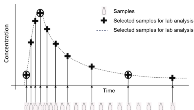
Figure 12 : Illustration of the correlation curve building comparing pollutant curve to wastewater samples
