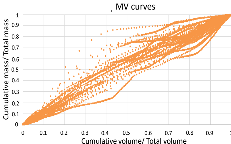
Figure 16 : Mass/Volume curves (Ly, 2019).
