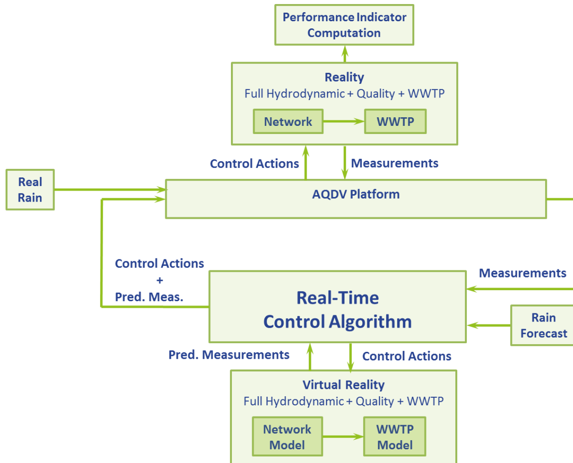
Figure 15 : Connection of the RTC CLSA with the AQDV platform in order to enable real testing to the PBRTC method.
