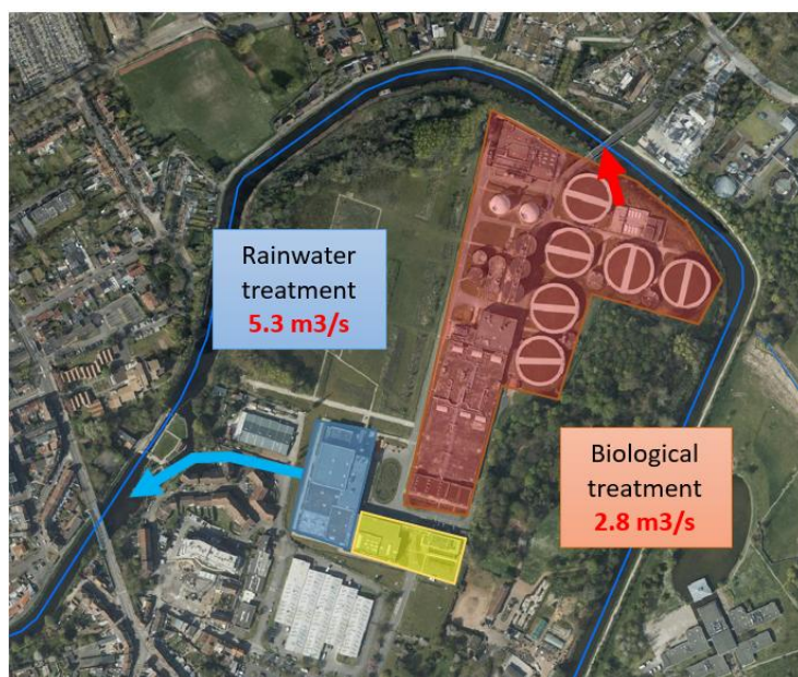
Figure 5 : Lille Marquette wastewater treatment plant - Biological treatment line - Rain treatment line - Discharge points to the canalized Marque river
