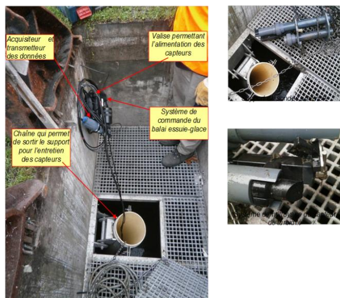
Figure 13 : Pictures illustrating the installation principle to be followed as the generic monitoring station set up (Maruéjols and Montserrat, 2016).
