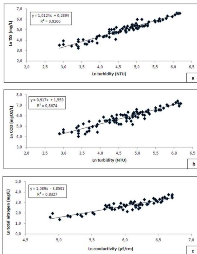
Figure 11 : Correlations between quality sensors (turbidity and conductivity) with classical pollutants (Bersinger et al., 2015)
