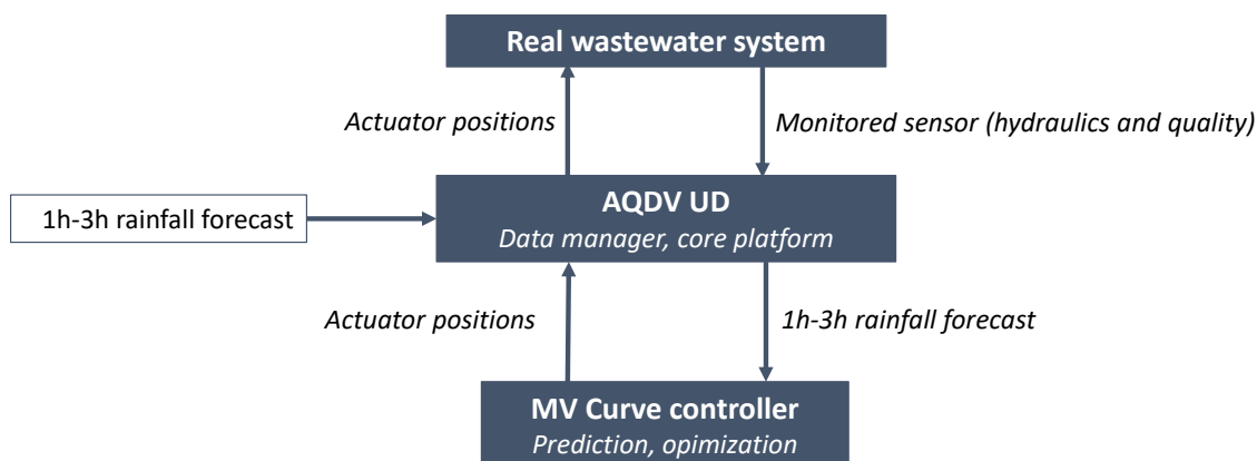
Figure 18 : Block diagram of closed-loop simulation scheme and integration with AQDV UD
