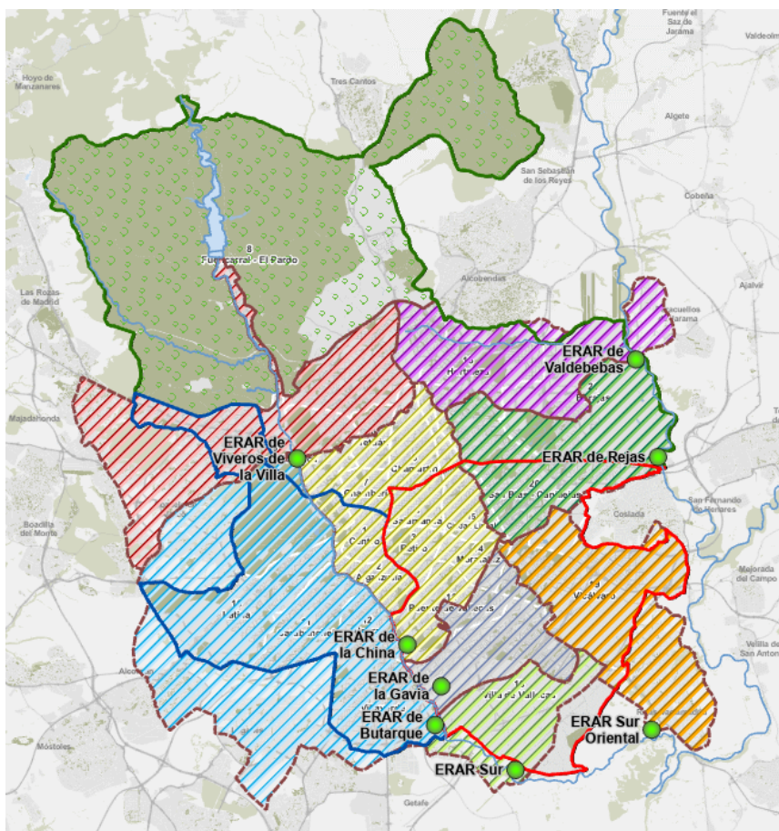
Figure 6 : Sewerage sub-basins of Madrid, linked to its main WWTP
