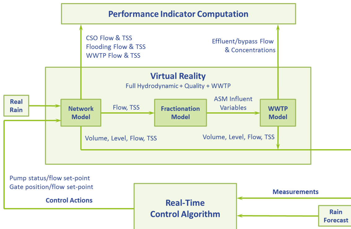
Figure 14 : Elements and variables taking part in a closed-loop simulation of RTC algorithm applied to integrated control of UDN and WWTP
