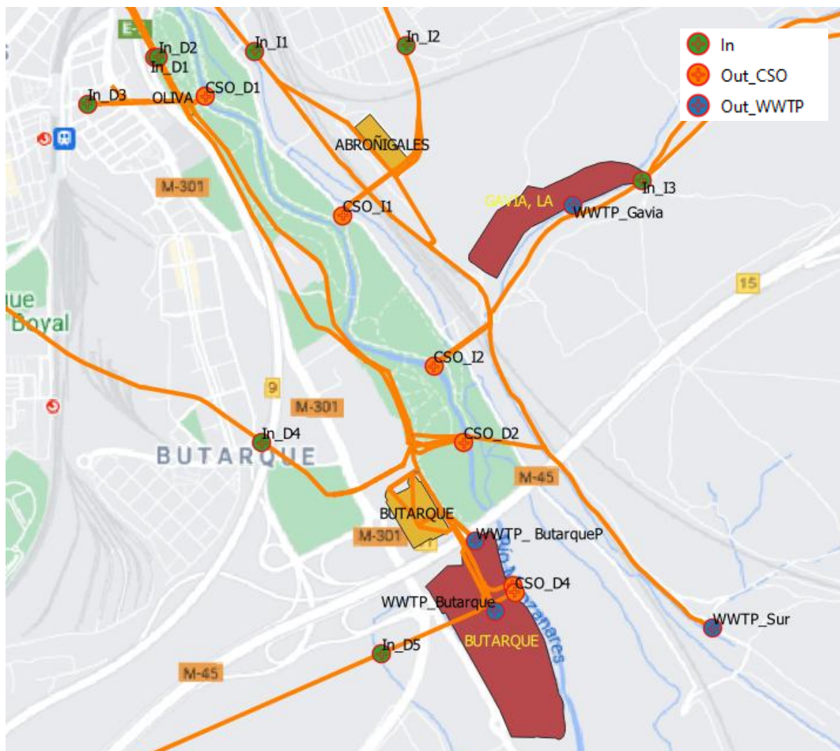
Figure 3 : Location of the flow inputs and output points in the pilot site
