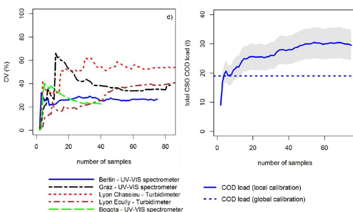
Figure 10 : Results from Caradot et al. (2014). On the left, the required number of samples to stabilise the coefficient of variation of quality sensor calibration. On the right, Comparison of total CSO COD load calculation using global and local calibration
