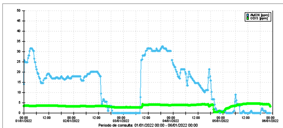
Figure 7 : Example of dissolved oxygen (green) and ammonium (blue) timeseries at Rivas Station downstream the site area (January-June 2022)
