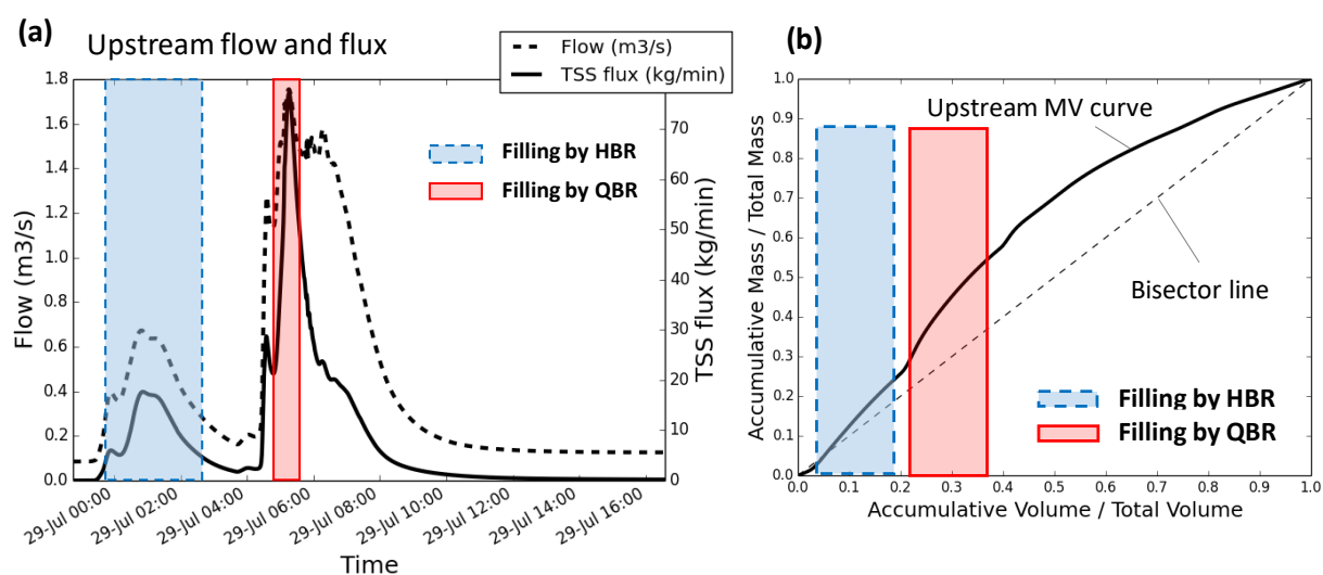
Figure 19 : a) Illustration of filling periods by two strategies overflow and TSS flux plots (upstream of the tank); b) Same illustration over the MV curve plot (upstream of the tank).
