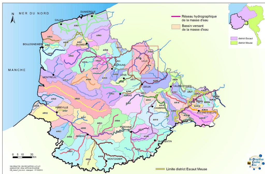
Figure 8 : Inland surface water bodies.
