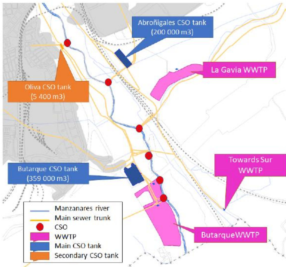
Figure 2 : Detail of the Rubies project pilot site in Manzanares system
