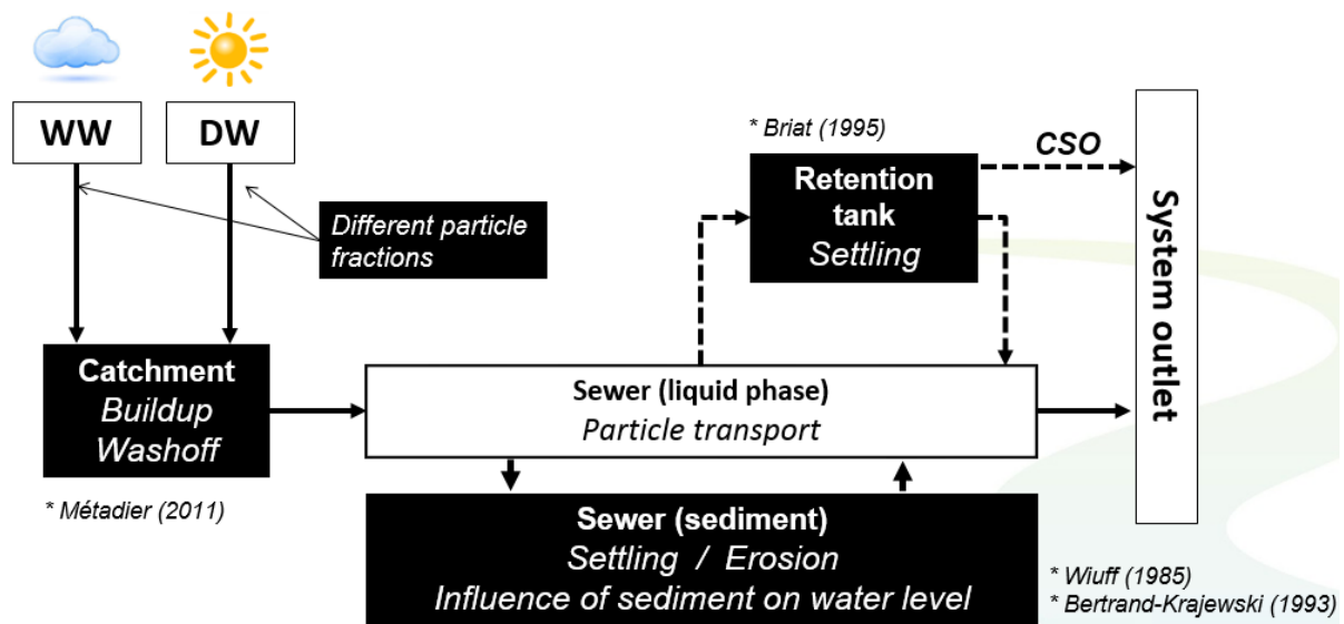
Figure 17 : Water quality processes included in the SWMM-TSS model (after Montserrat et al., (2017)). Black boxes indicate the processes improved by the new library, with given references for the used equations.
