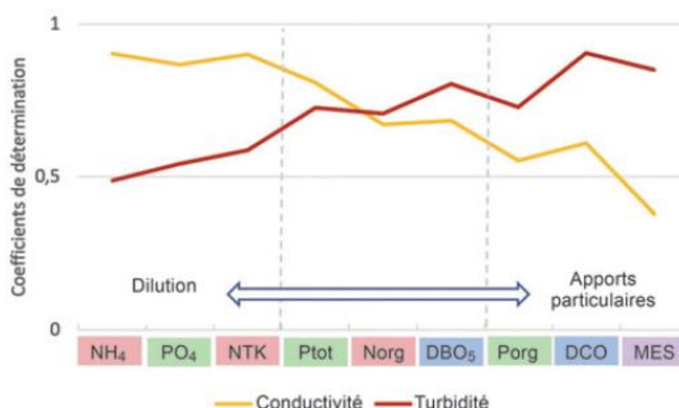
Figure 9 : Correlations between quality sensors (turbidity and conductivity) with classical pollutants (Patris et al., 2020)
