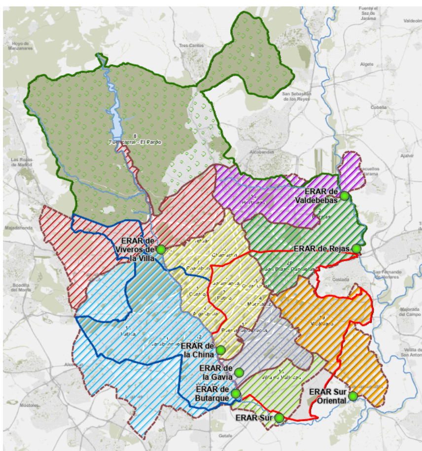
Figure 64.- Sewerage sub-basins of Madrid, linked to its main WWTP.
