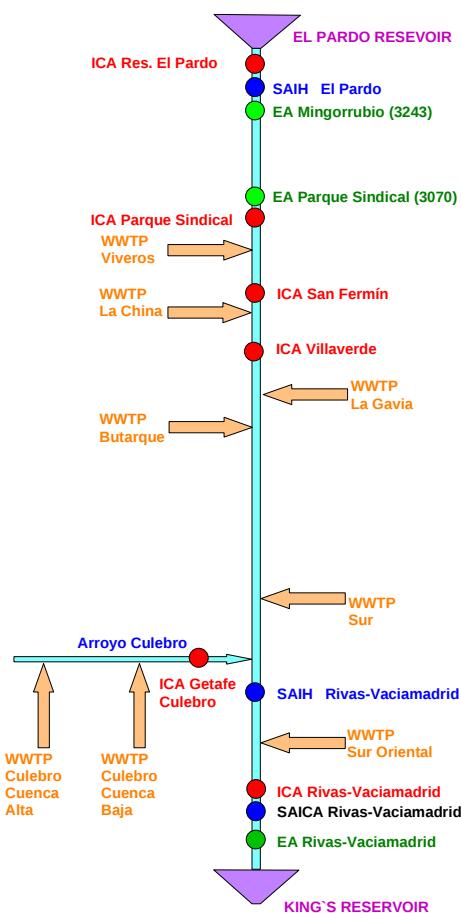
Figure 68.- Sketch showing the location of the WWTPs and the water quality and flow control stations.
