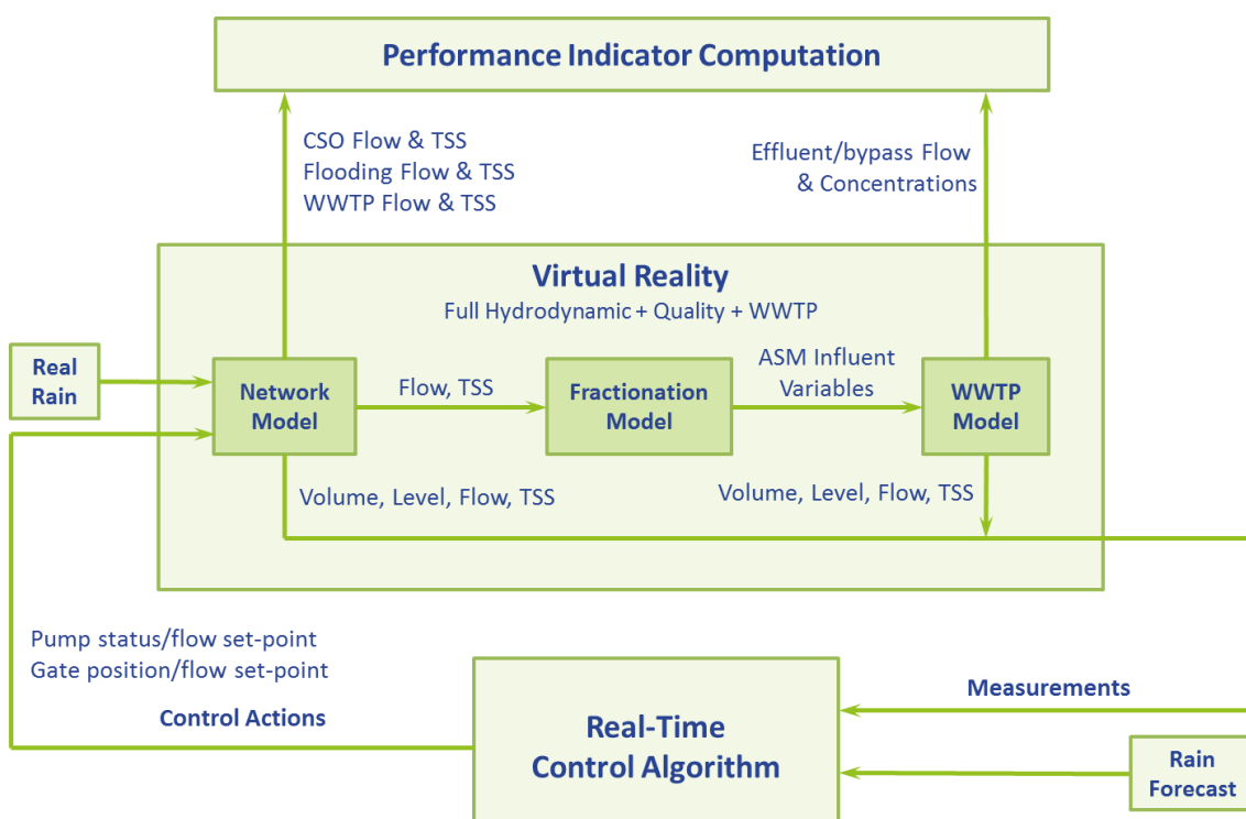
Figure 58.- Elements and variables taking part in a closed-loop simulation of RTC algorithm applied to integrated control of UDN and WWTP.
