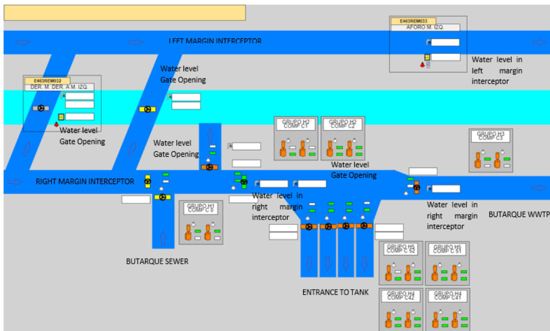
Figure 30.- Connections between left and right bank interceptors and diversion to Butarque tank
