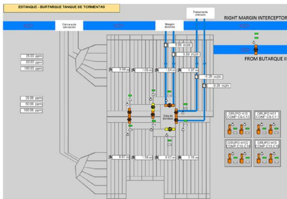
Figure 34.- Sensor monitoring in the tank's compartments and pumping station
