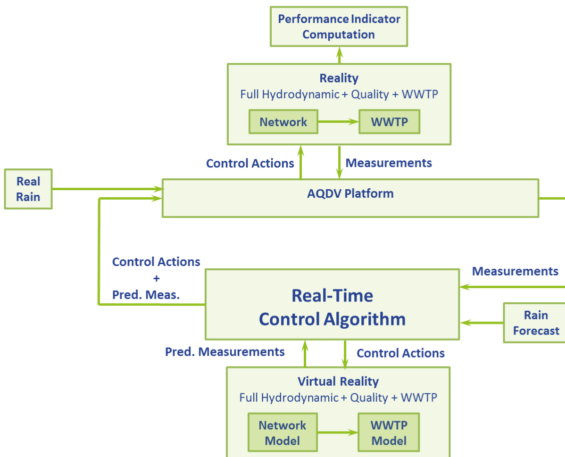
Figure 60: Connection of the RTC CLSA with the AQDV platform in order to enable real testing to the PBRTC method.
