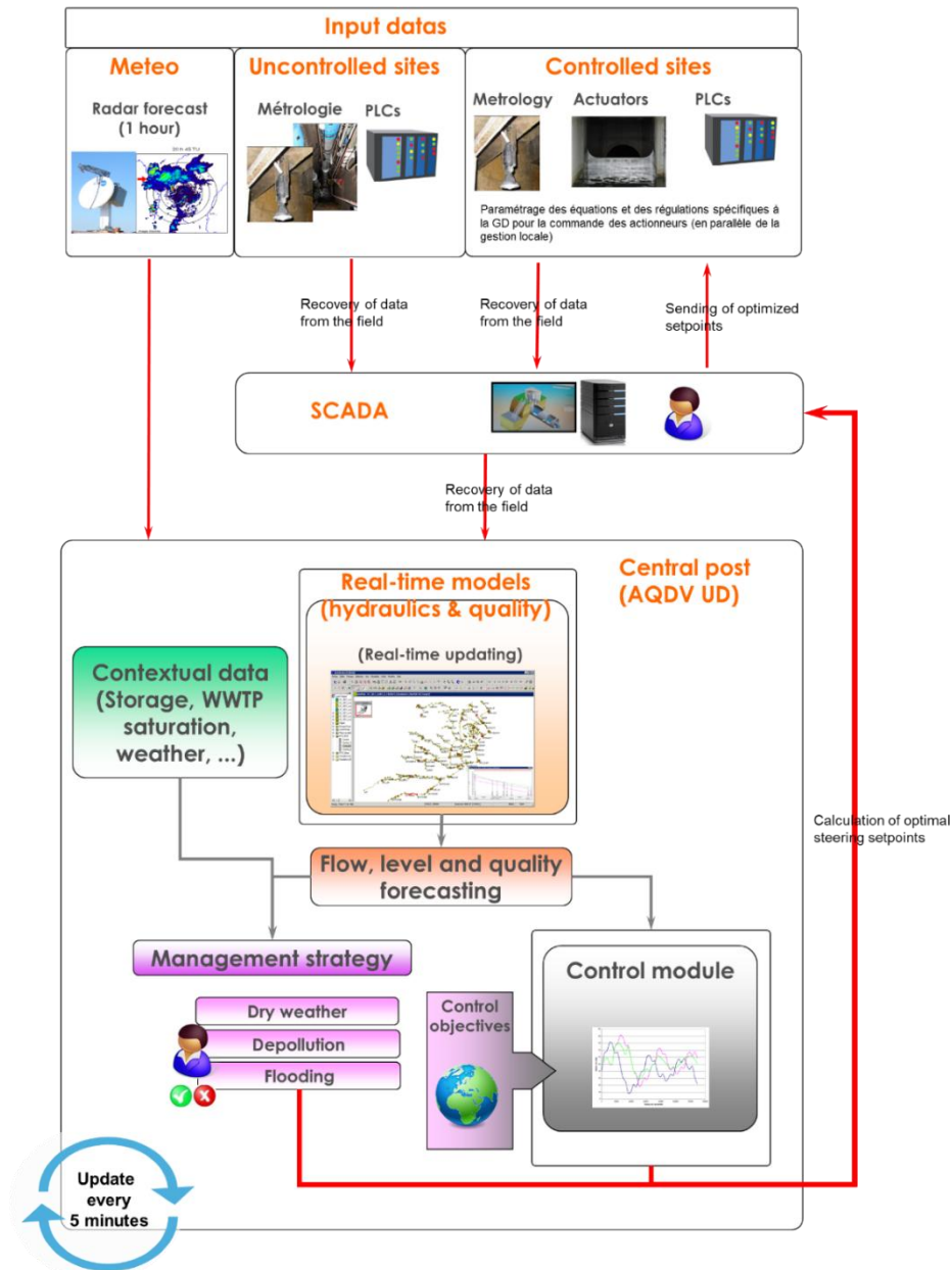
Figure 55.- AQDV UD connection with the Canal Isabel II IT system
