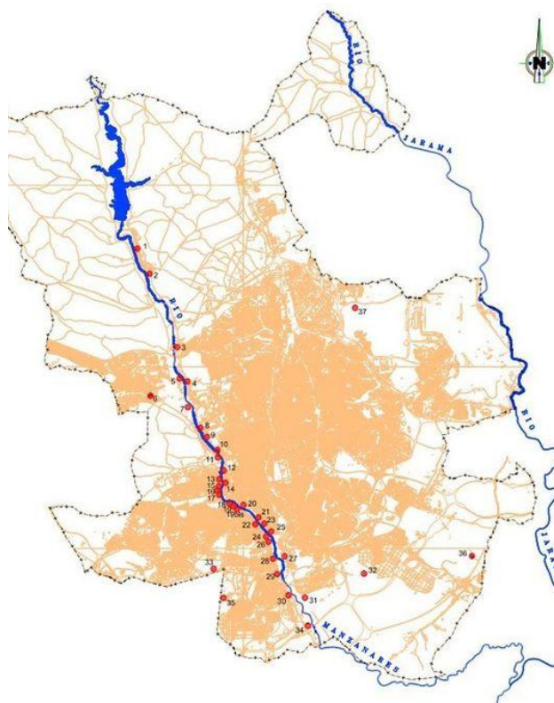
Figure 65.- CSO discharge points on the Manzanares River.
