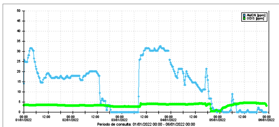
Figure 70.- Example of dissolved oxygen (green) and ammonium (blue) timeseries at Rivas Station (January-June 2022)
