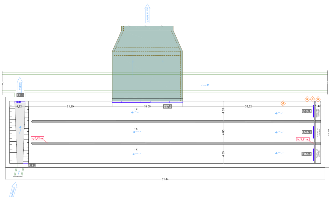
Figure 5.- Horizontal plan and dimensions of the Oliva tank and the location of the gate connecting the tank with the right margin interceptor.
