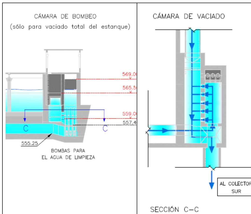
Figure 16.- Cross section (left) and horizontal map (right) of the emptying chamber and the the pumping station
