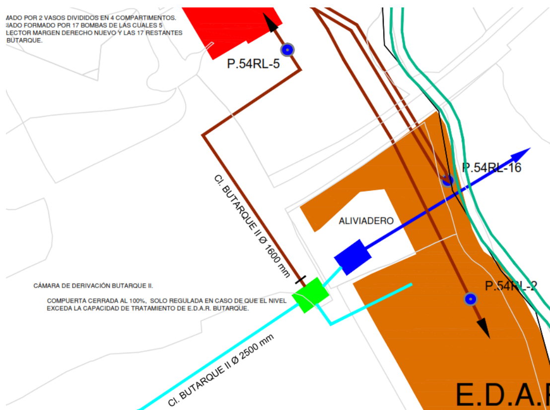
Figure 9.- Butarque II tributary sewer and its connection to the tank, WWTP and CSO discharging point
