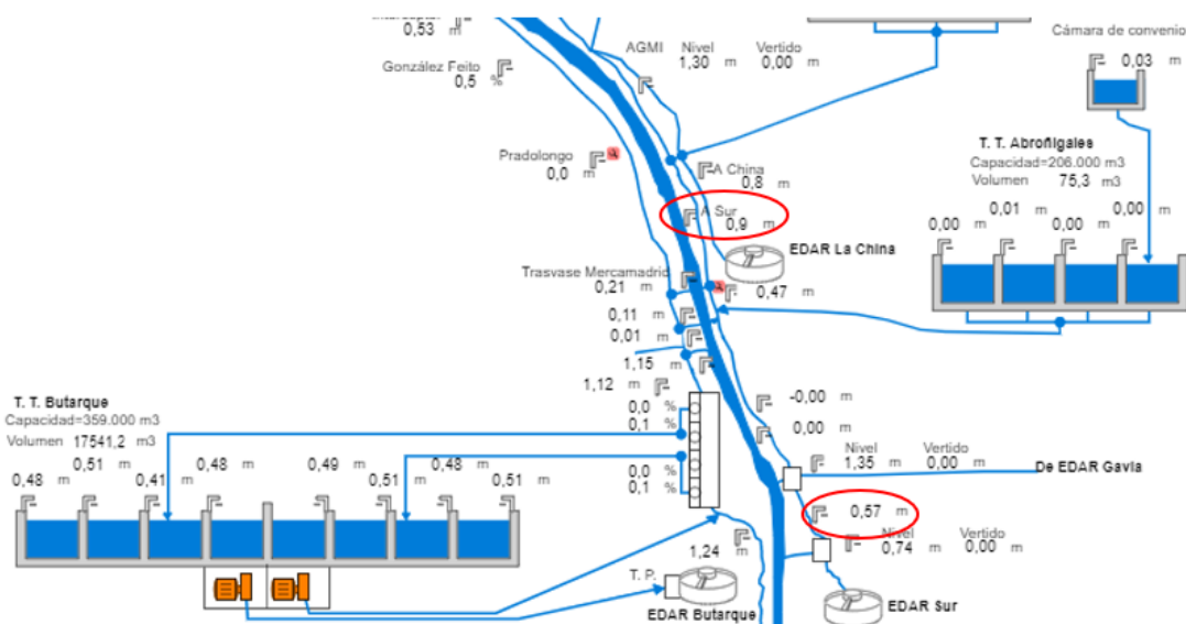
Figure 29.- Water level sensors located within the study area
