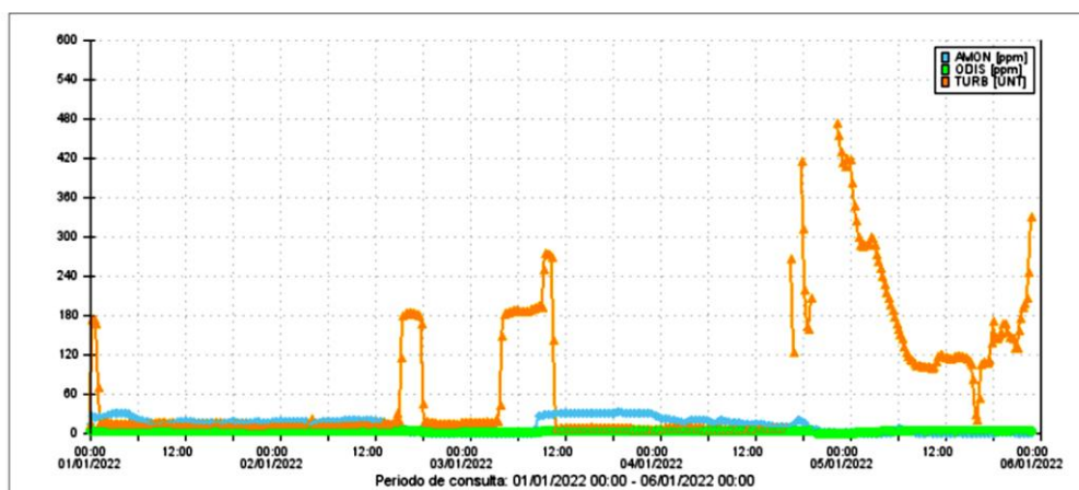
Figure 71.- Example of dissolved oxygen (green), ammonium (blue) and turbidity (orange) timeseries at Rivas Station (January-June 2022)
