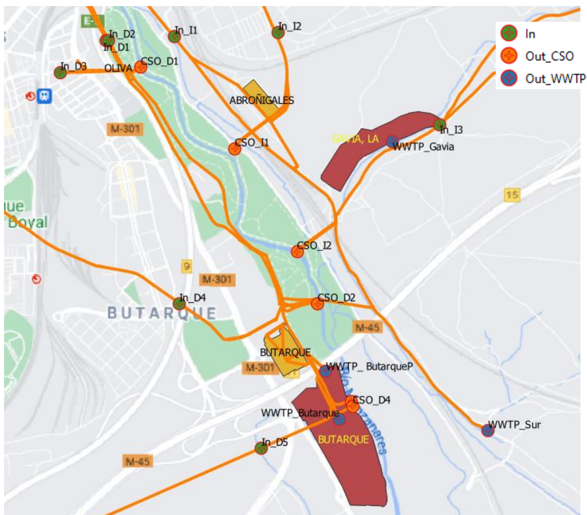
Figure 3.- Location of the flow inputs and output points in the pilot site
