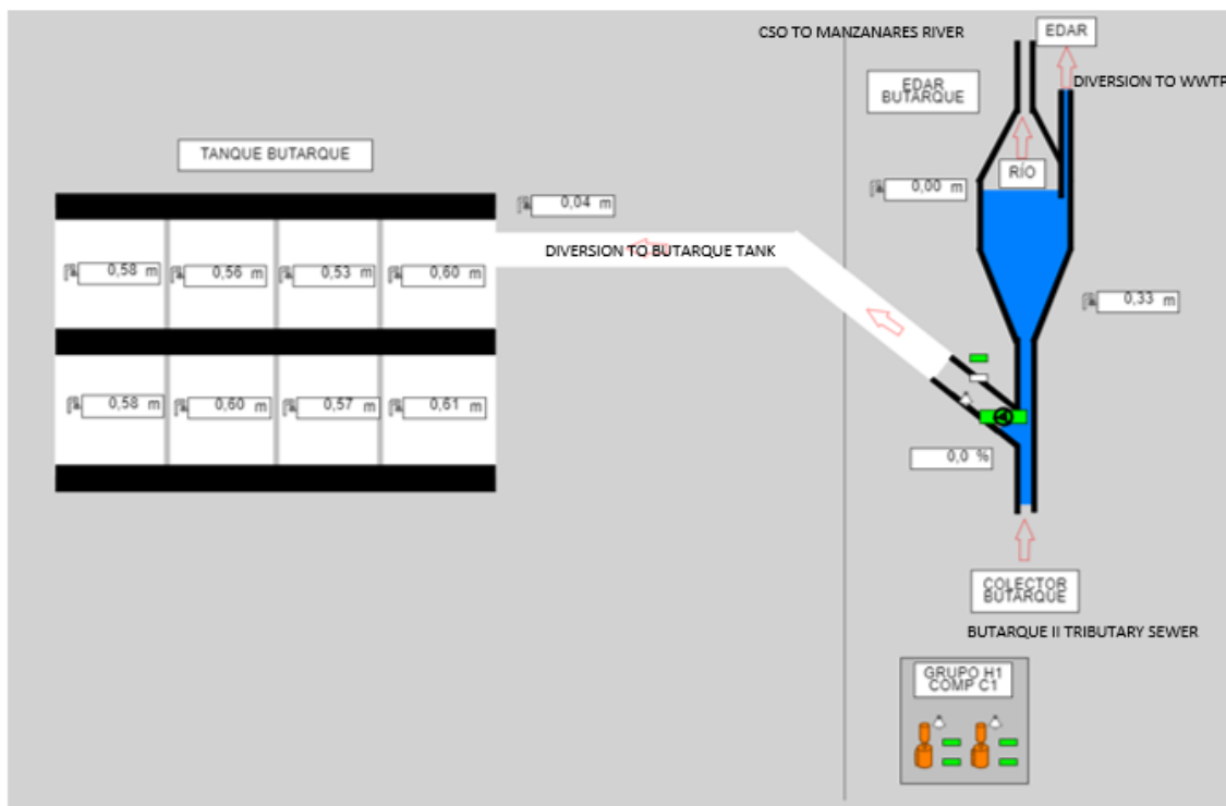
Figure 31.- Diversion point at the end of Butarque II tributary sewer
