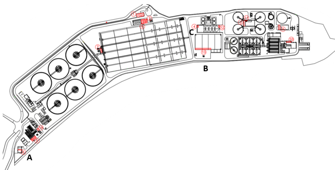
Figure 38.- Plan view of La Gavia WWTP with reference to the existing gauges and weirs
