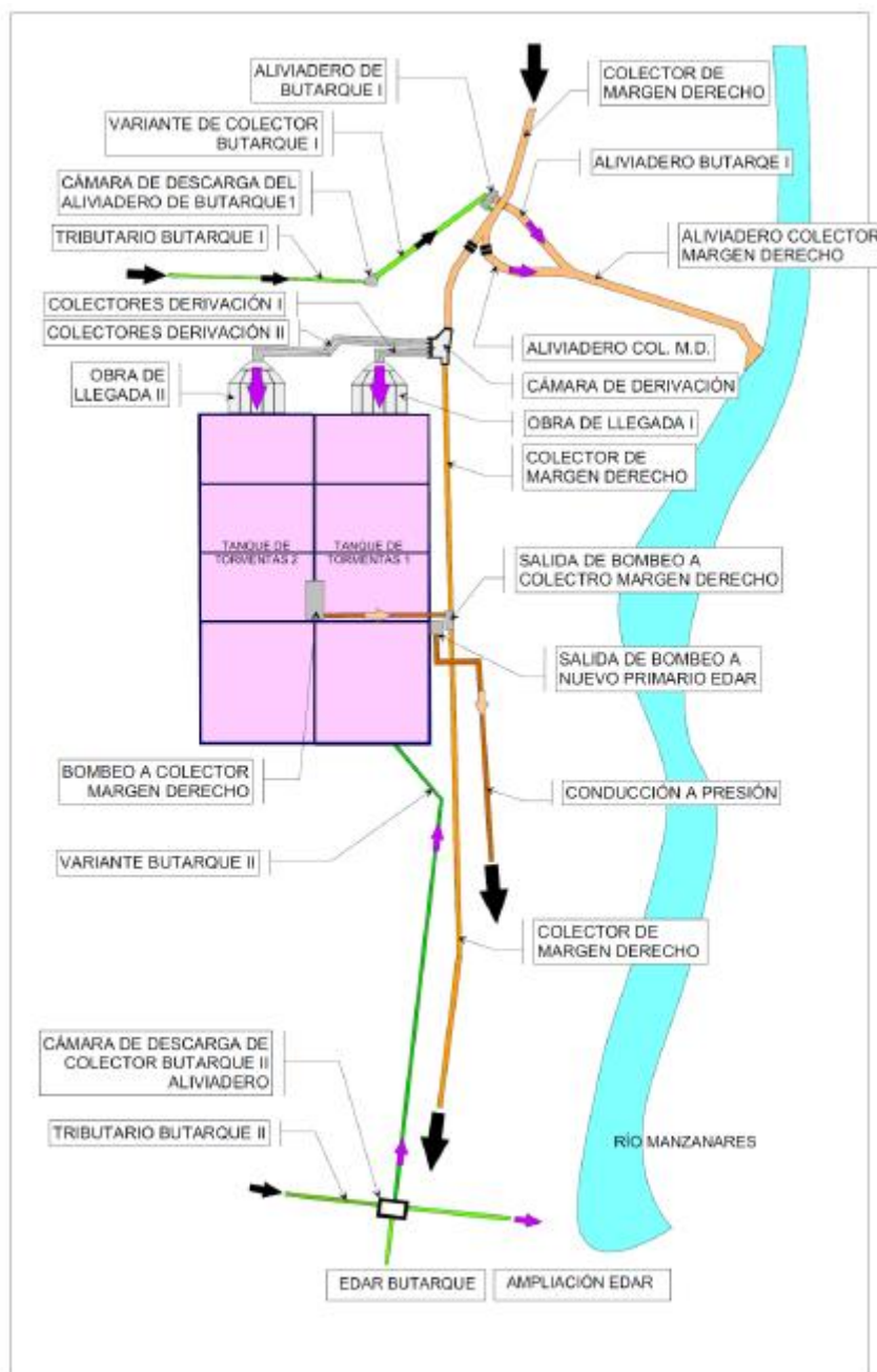
Figure 8.- Main sewers and infrastructures around Butarque tank
