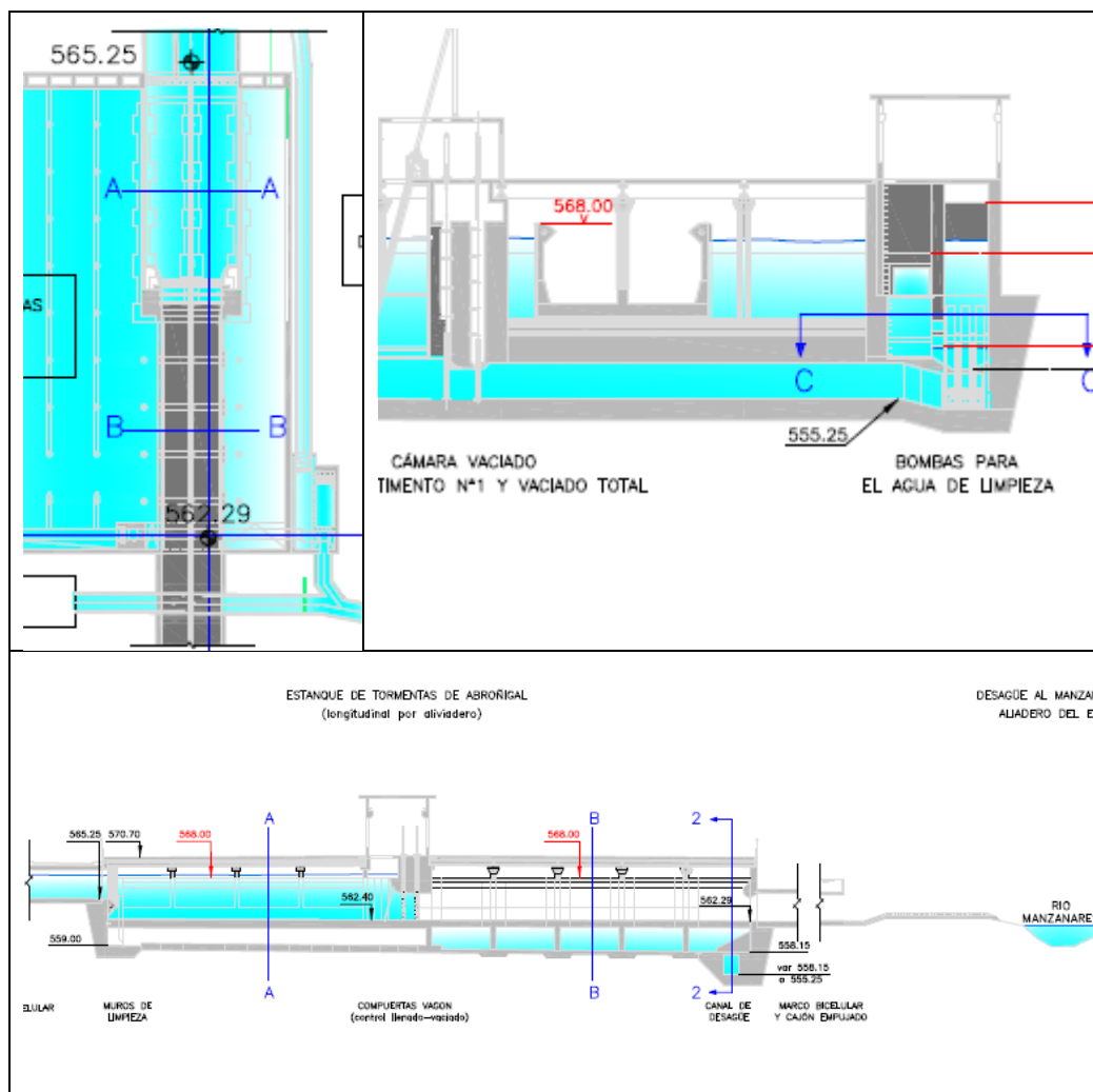
Figure 14.- Horizontal plan longitudinal and cross section of the channel
