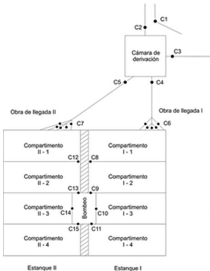
Figure 32.- Schematic view of Butarque tank partitioning
