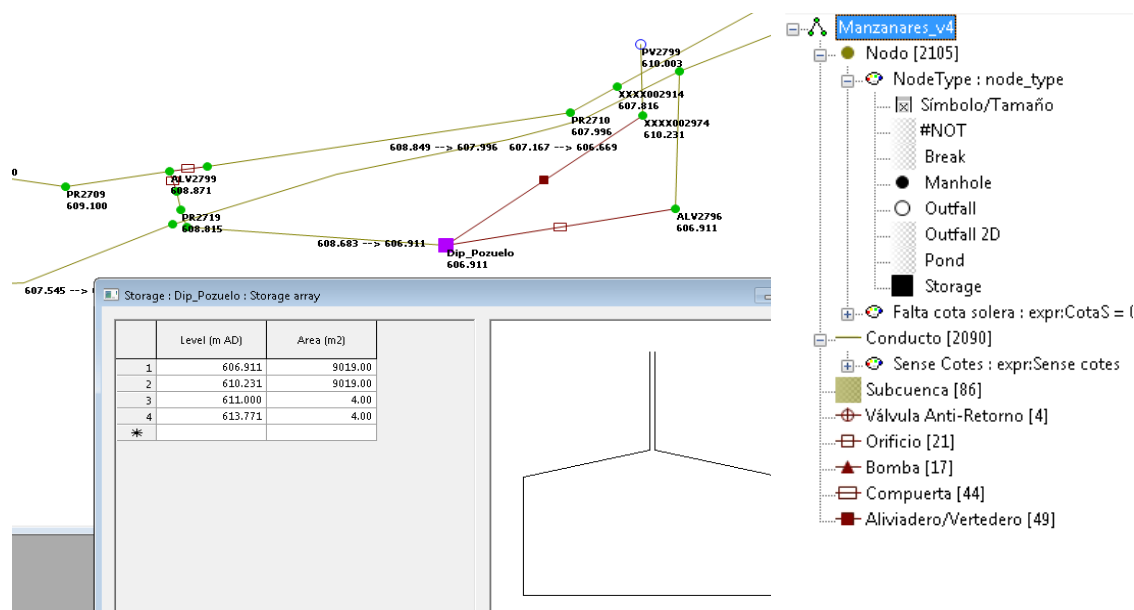
Figure 40.- Example of detention tank model configuration
