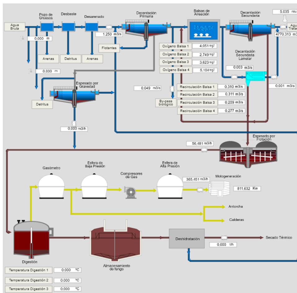
Figure 10.- Overall layout of Butarque WWTP
