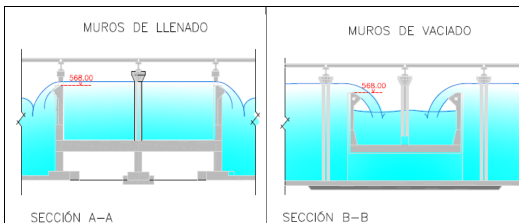
Figure 15.- Filling the tank with the channel gates closed (left). Emptying the tank through the emergency weirs once the tank is full (right).
