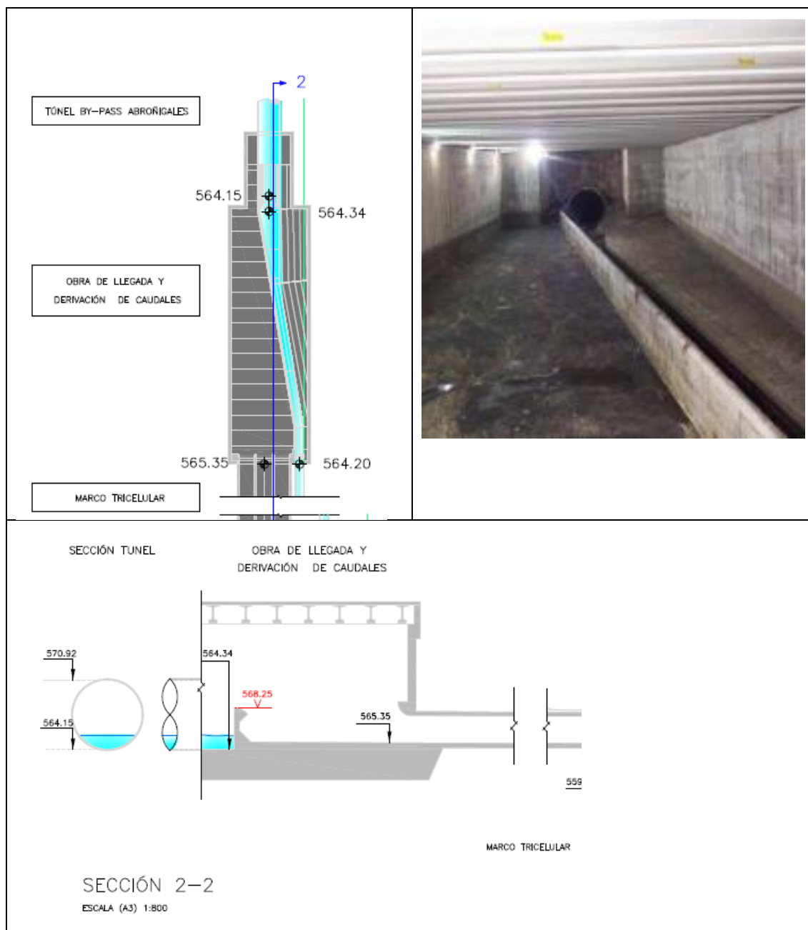
Figure 13.- Scheme and photo of the entrance diversion chamber to Abroñigales tank
