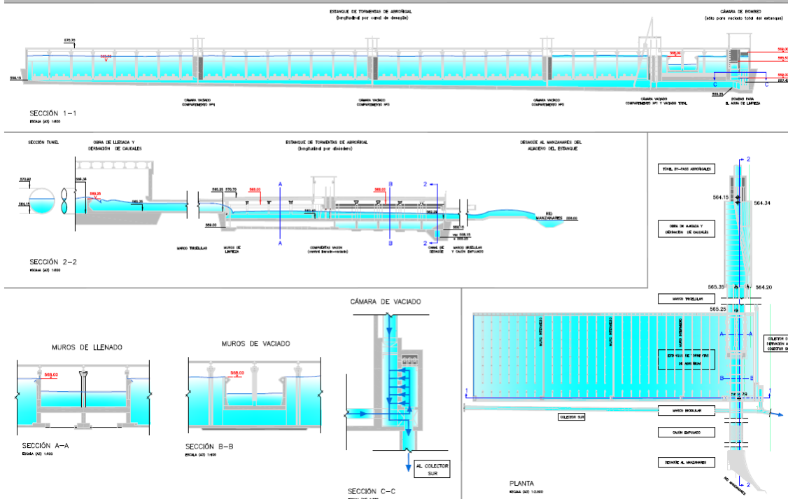
Figure 19.- Abroñigales operation model for case 3
