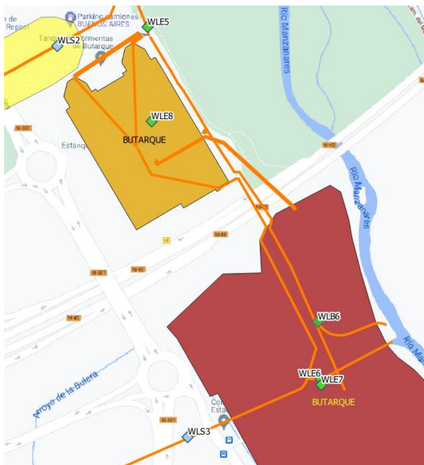
Figure 53.- Location of WLS2 and 3 located in the collectors Butarque I and Butarque II
