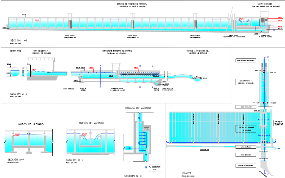
Figure 20.- Abroñigales operation model for case 4
