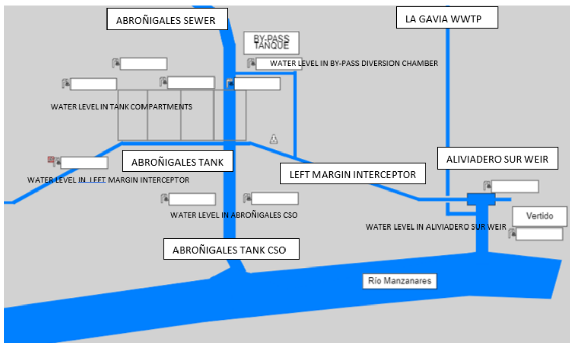
Figure 36.-Schematic view of the Abroñigales system with reference to the existing sensors in gauges and weirs
