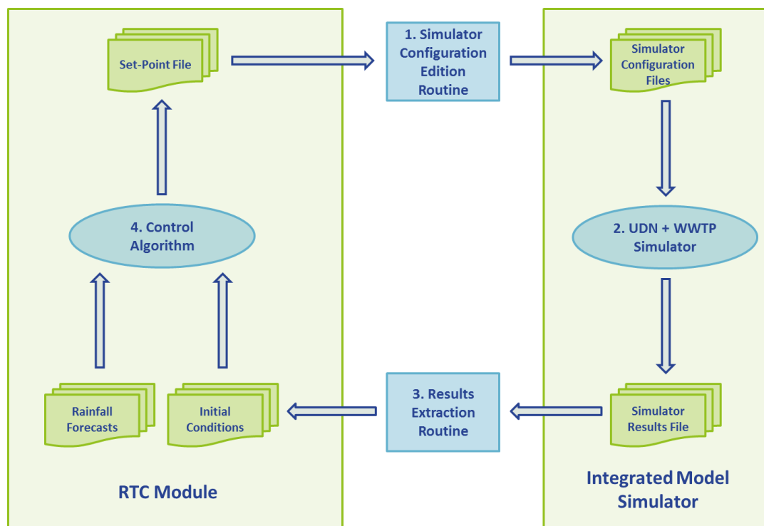
Figure 59: CLSA implementation steps and information flow between a virtual reality simulator and a real-time controller.
