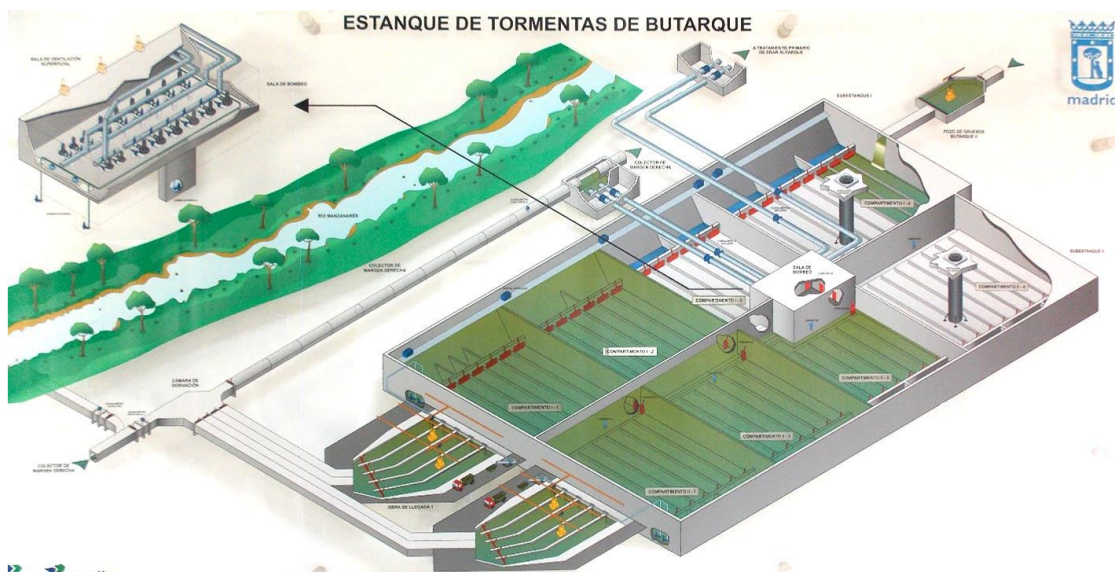
Figure 7.- General scheme of Butarque CSO tank.
