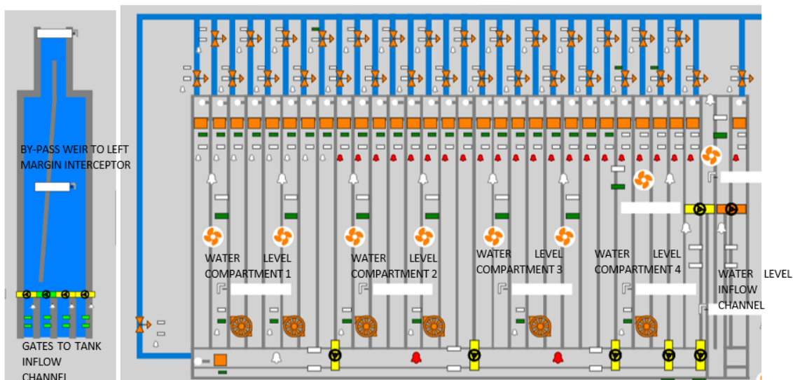
Figure 37.- Existing monitoring signals inside Abroñigales tank
