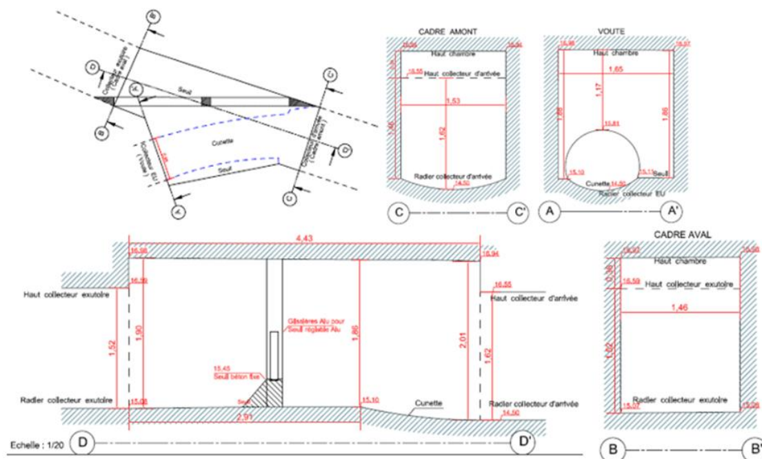
Figure 31 : Design schematics of Saint Hélène Pasteur weir
