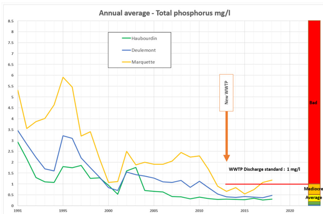
Figure 14 : Average river phosphorus over the years
