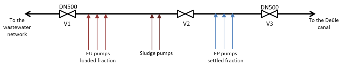
Figure 22 : Automatic operation mode schematic
