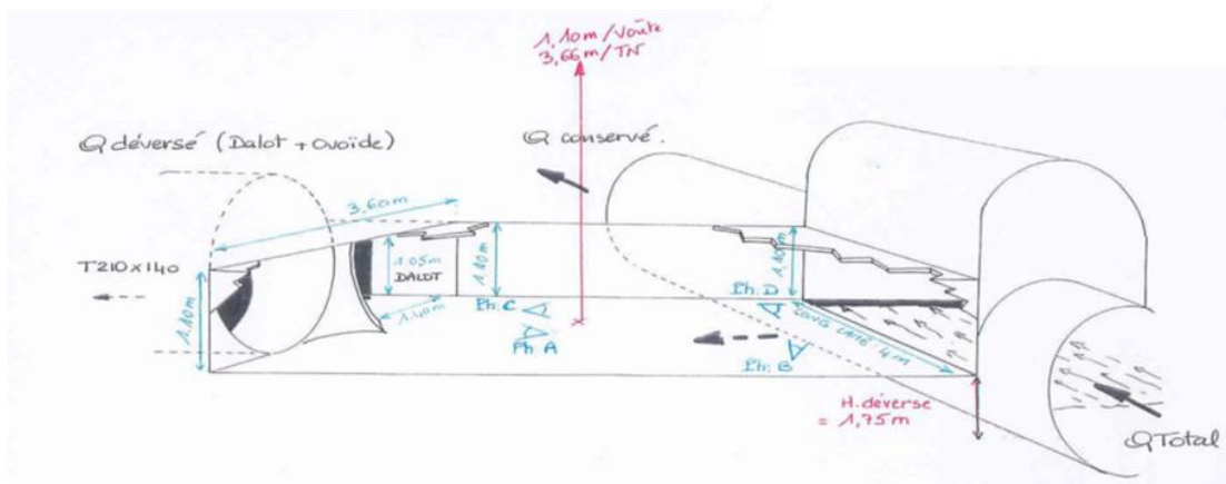
Figure 18 : Sketch of the Denis du Péage weir
