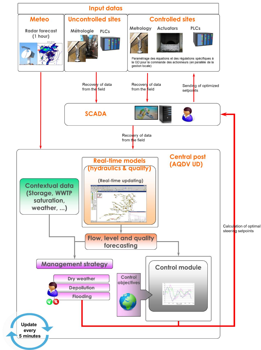
Figure 54 : AQDV UD infrastructure schematic
