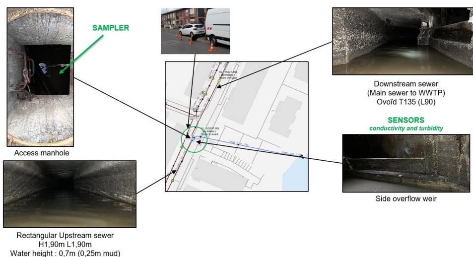
Figure 46 : Sainte Hélène/Thiers monitoring station GIS location and sewer pictures
