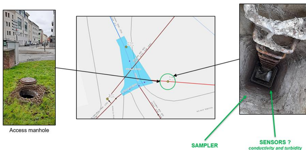
Figure 51 : Maracci's site 2 monitoring station GIS location and sewer pictures
