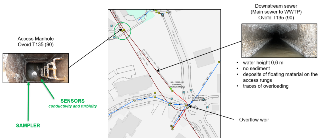
Figure 47 : Sainte Hélène/Pasteur monitoring station GIS location and sewer pictures
