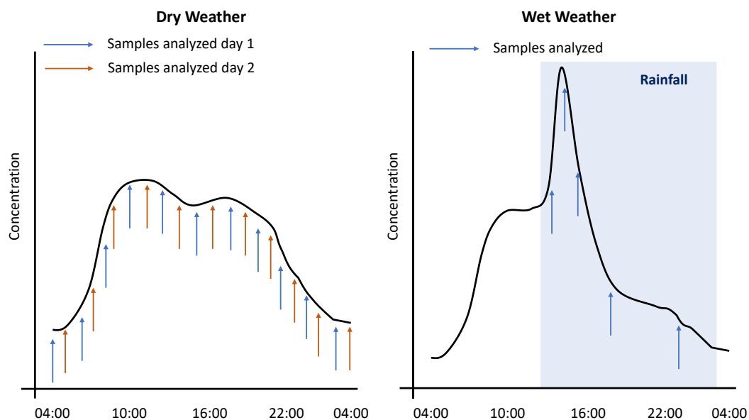
Figure 53 : Sampling strategy for quality sensor in situ calibration
