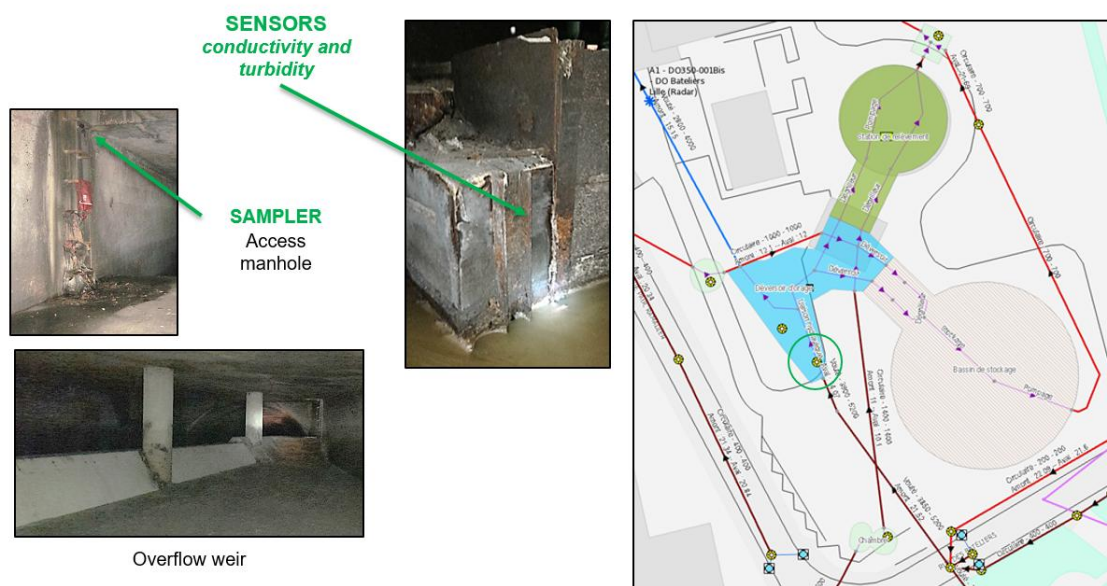
Figure 49 : Bateliers monitoring station GIS location and sewer pictures
