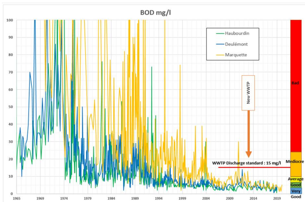
Figure 7 : River BOD over the years
