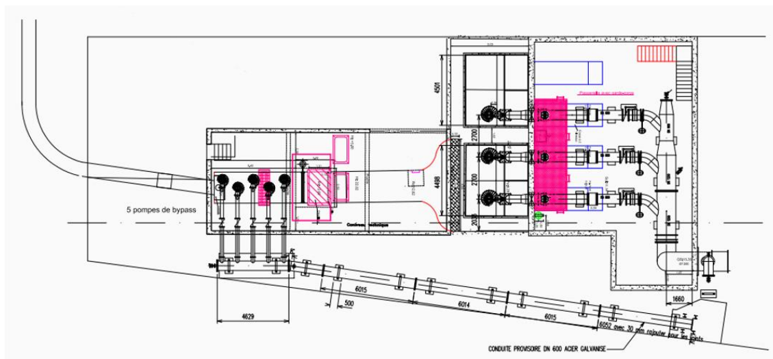
Figure 32 : Pont Abbaye Pumping station – Plan view
