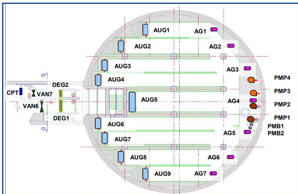
Figure 35 : Plan view of the basin.
