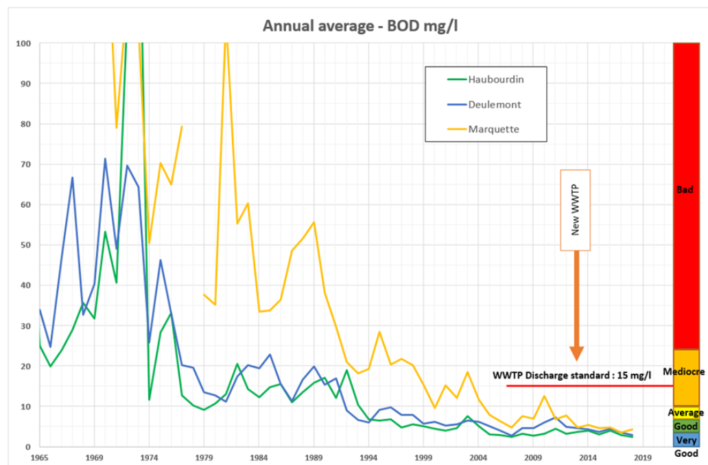
Figure 8 : Average river BOD over the years
