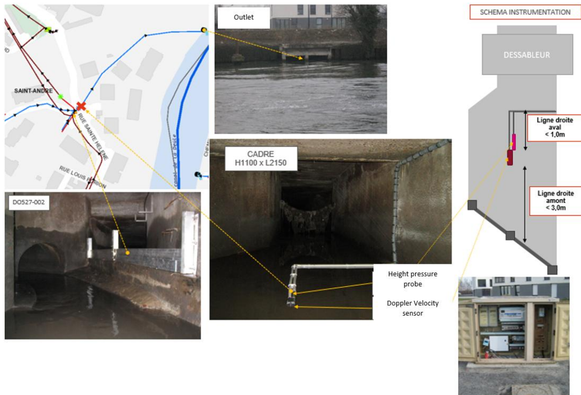
Figure 30 : Illustrations of Saint Hélène Pasteur weir
