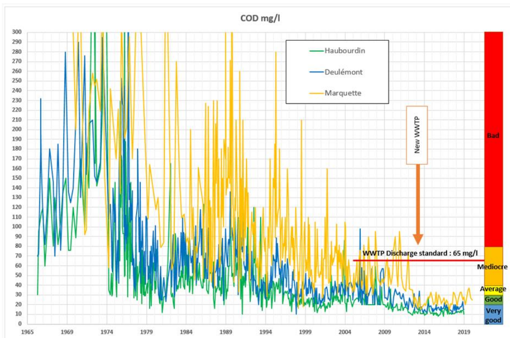
Figure 9 : River COD over the years
