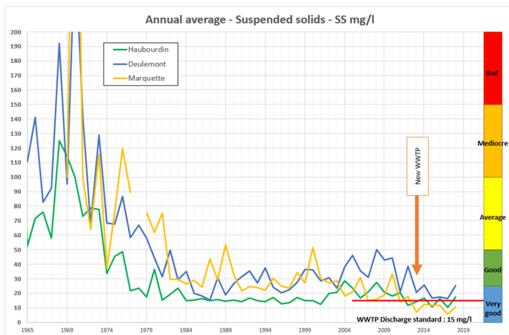
Figure 6 : River average suspended solids over the years
