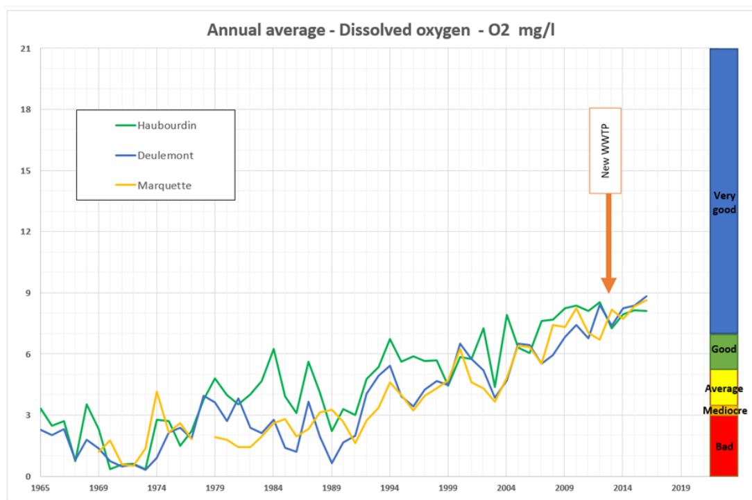
Figure 15 : River DO over the years
