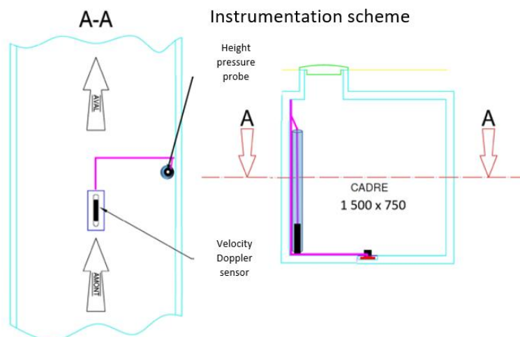
Figure 19 : Denis du Péage instrumentation scheme
