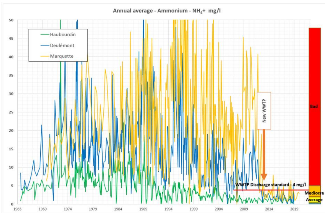
Figure 11 : River NH4 over the years
