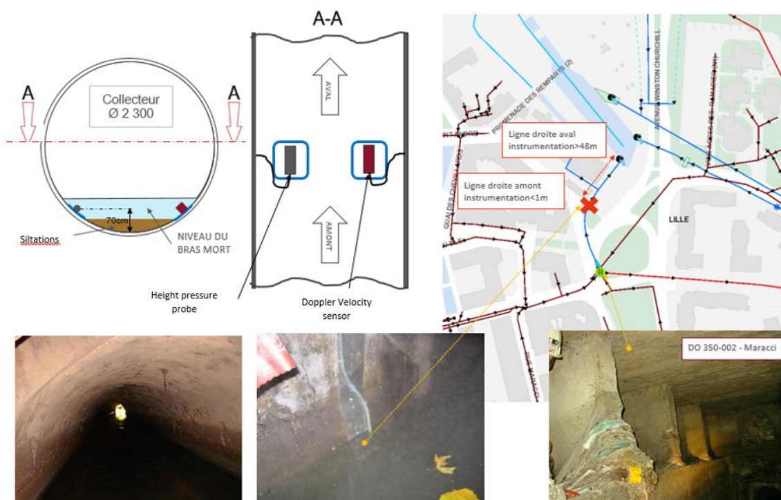
Figure 38 : Illustrations of Maracci's weir
