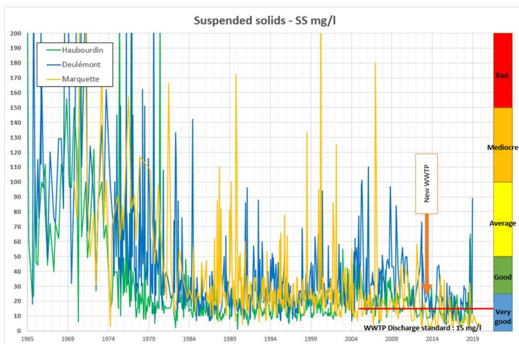
Figure 5 : River suspended solids over the years
