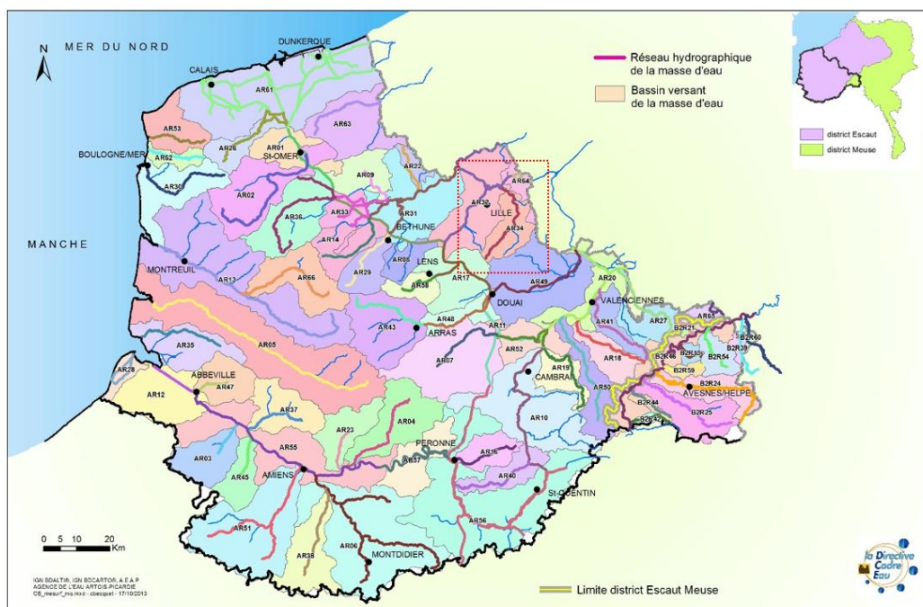
Figure 3 : Inland surface water body
