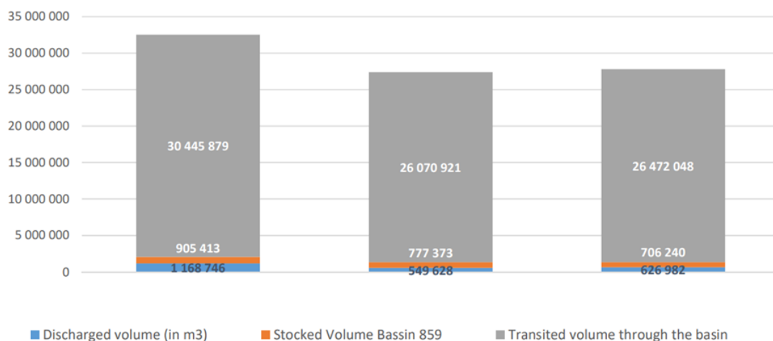
Figure 40 : Bateliers basin – Interannual evolution since 2019
