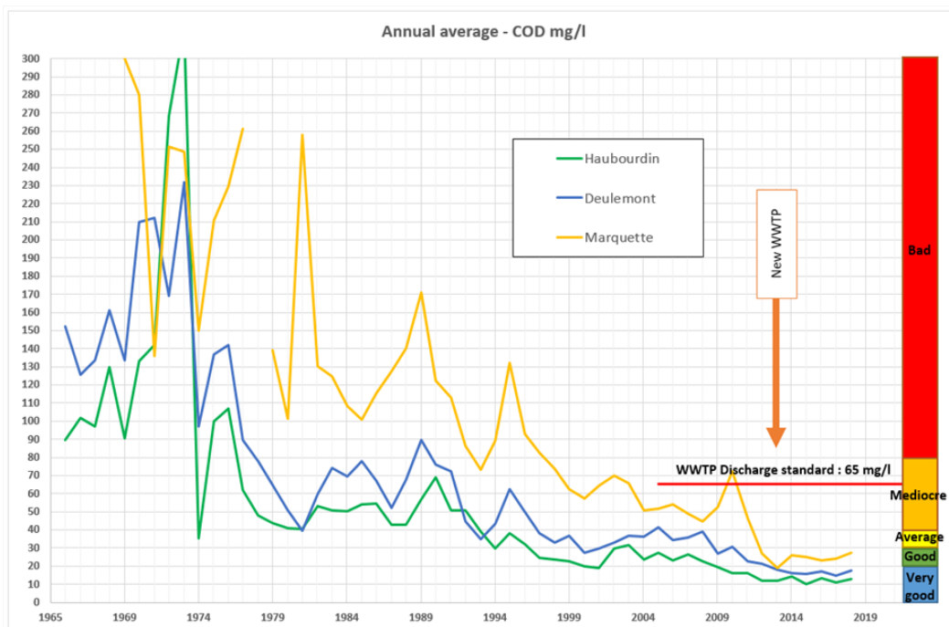
Figure 10 : Average river COD over the years
