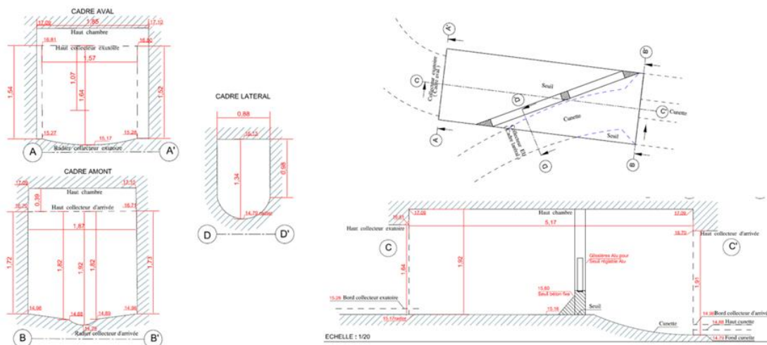
Figure 29 : Design schematics of Saint Hélène Thiers weir
