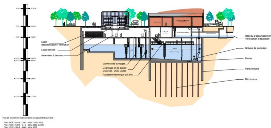
Figure 34 : Connection structure to the WWTP
