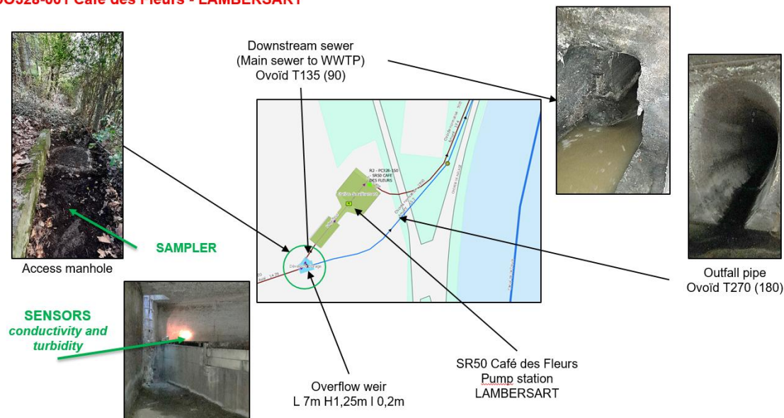
Figure 48 : Café des fleurs monitoring station GIS location and sewer pictures
