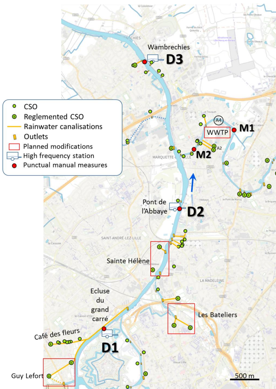
Figure 61 : Study site with the predicted instrumentation locations
