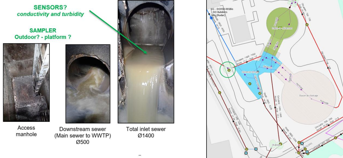
Figure 50 : Maracci's site 1 monitoring station GIS location and sewer pictures
