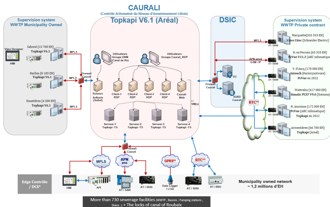
Figure 45 : OT/IT – supervision system of DEA (Water and Sewerage department)
