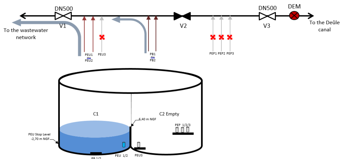
Figure 23 : Pollution mode - Phase 1 schematic
