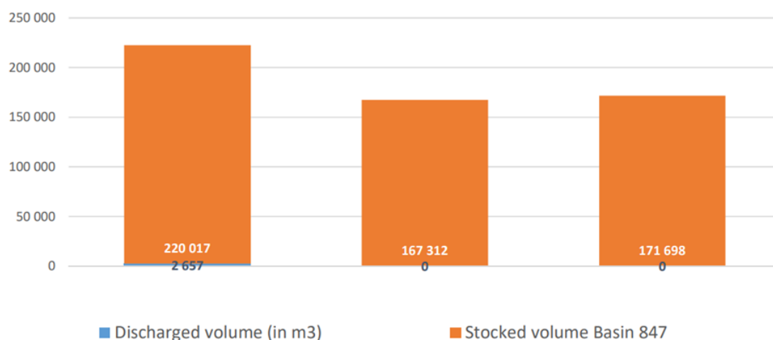
Figure 41 : Guy Lefort basin – Interannual evolution since 2019
