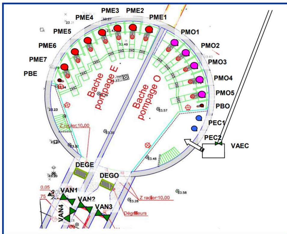
Figure 33 : Plan view of the pumping station
