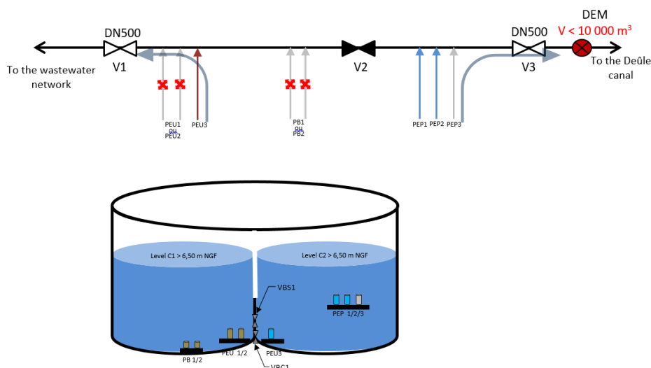
Figure 25 : Flooding mode with High level - Phase 1 schematic
