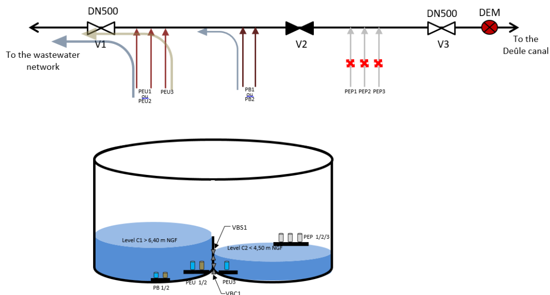
Figure 24 : Flooding mode with Low level - Phase 1 schematic
