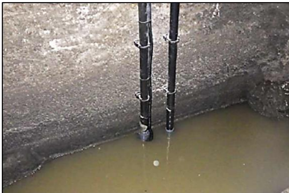
Figure 12 Sensors installed in the sewer of weir 328-001
