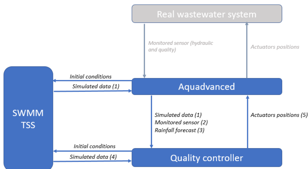
Figure 23 - Block diagram of closed-loop simulation scheme and integration with AQDV UD
