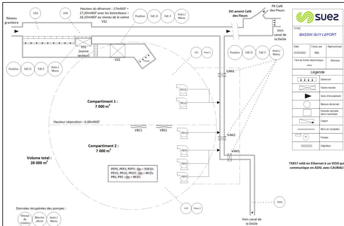
Figure 27 : Instrumentation diagram of Guy Lefort storm water tank
