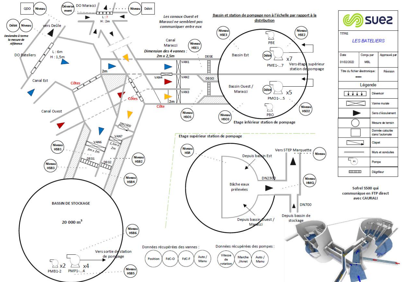
Figure 28 : Instrumentation diagram of Bâteliers storm water tank
