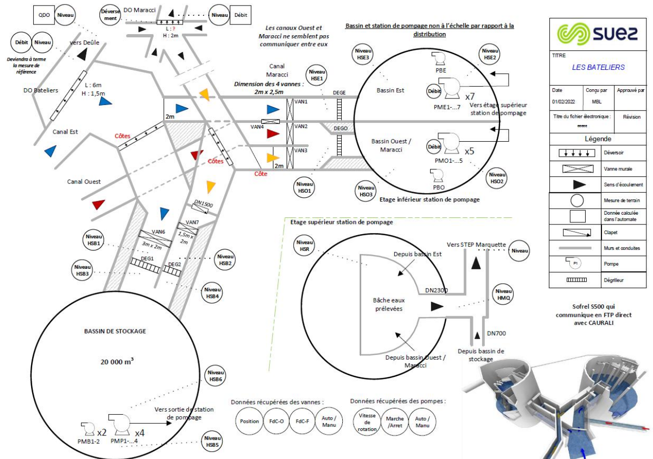
Figure 29 : Instrumentation diagram of Café des fleurs storm water tank
